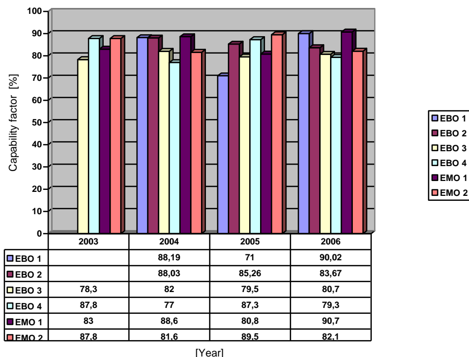
Obr. 6.1.1 Unit capability factor
