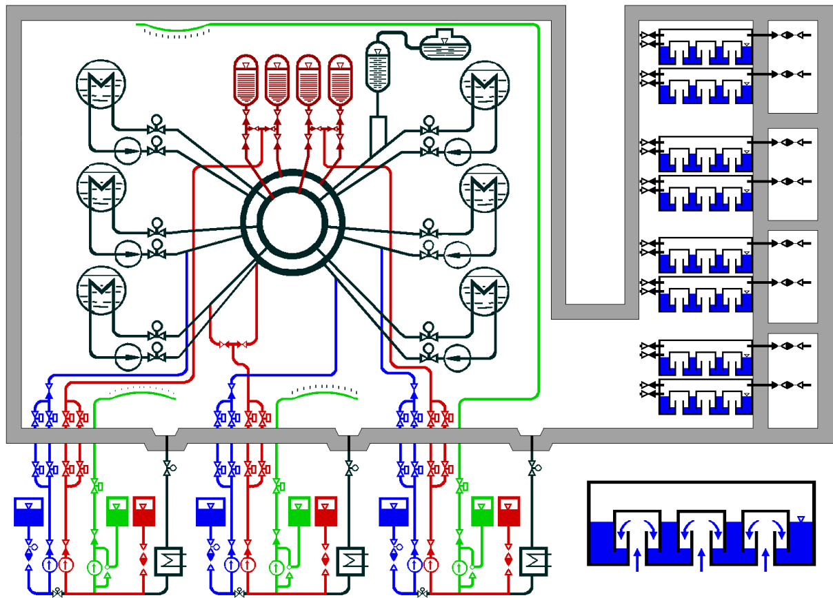
Figure No. 2.2.1 Safety systems of WWER 440 units - model V 213
