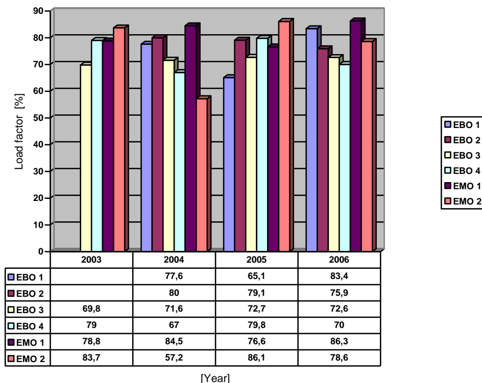
Pict. 6.1.2 Units SE-EBO and SE-EMO load factor
