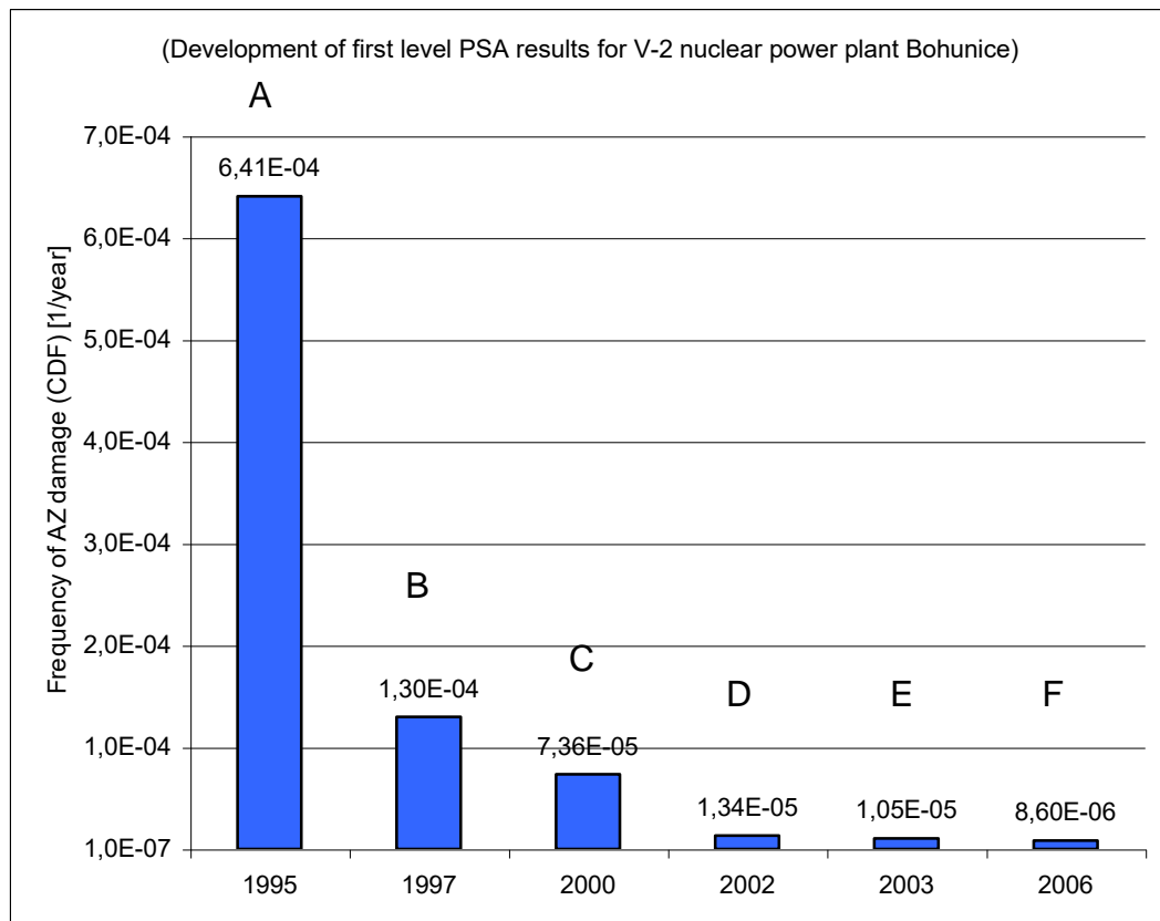
Figure No. 2.2.2 Development of Level 1 PSA results for V-2 nuclear power plant Bohunice
